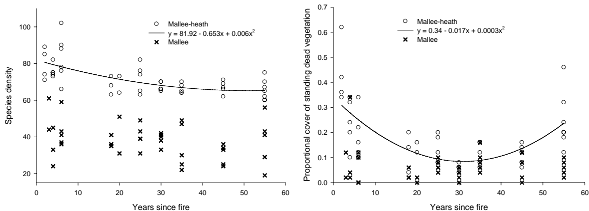
Fig. 1. Relationships in mallee and mallee-heath between the number of years since fire and (left) the number of species per 100m 2 , and (right) the proportion of point intercepts with standing dead vegetation. Regression curves are shown, with no significant relationship in the mallee community in either case.
